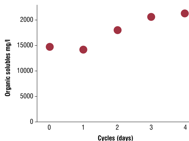
Figure 1: Levelling of organic solubles in recovered float vs time
