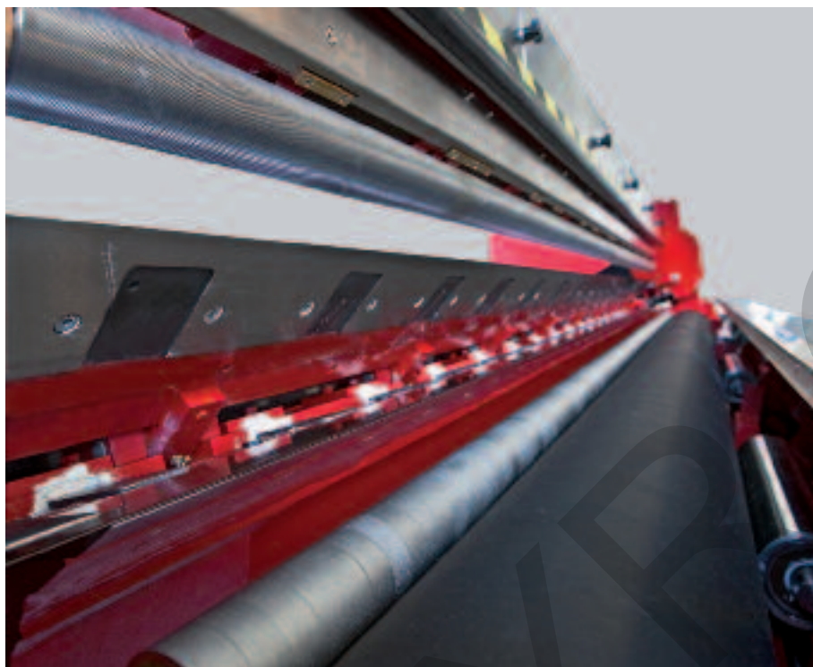
Machine opened with band knife shielded. The special elements of the Lintasplit machine have been retained and refined by Gemata.
